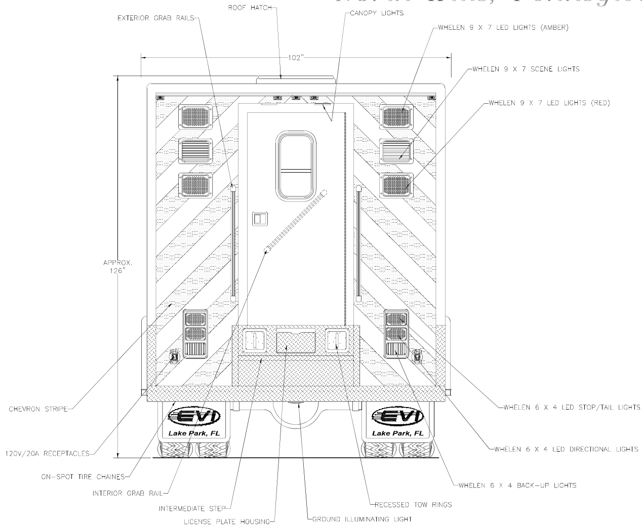
Rear View
