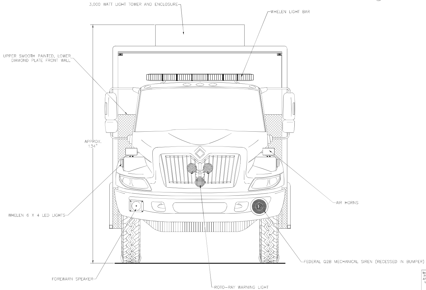
Front View
