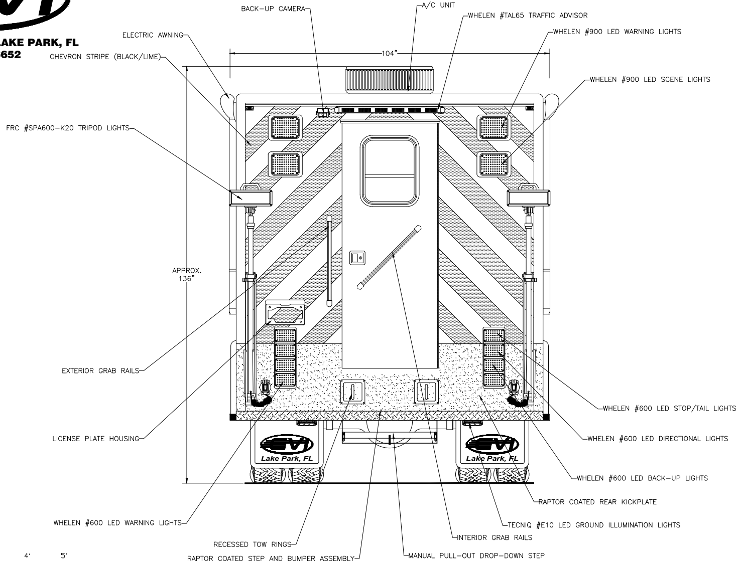
Rear View
