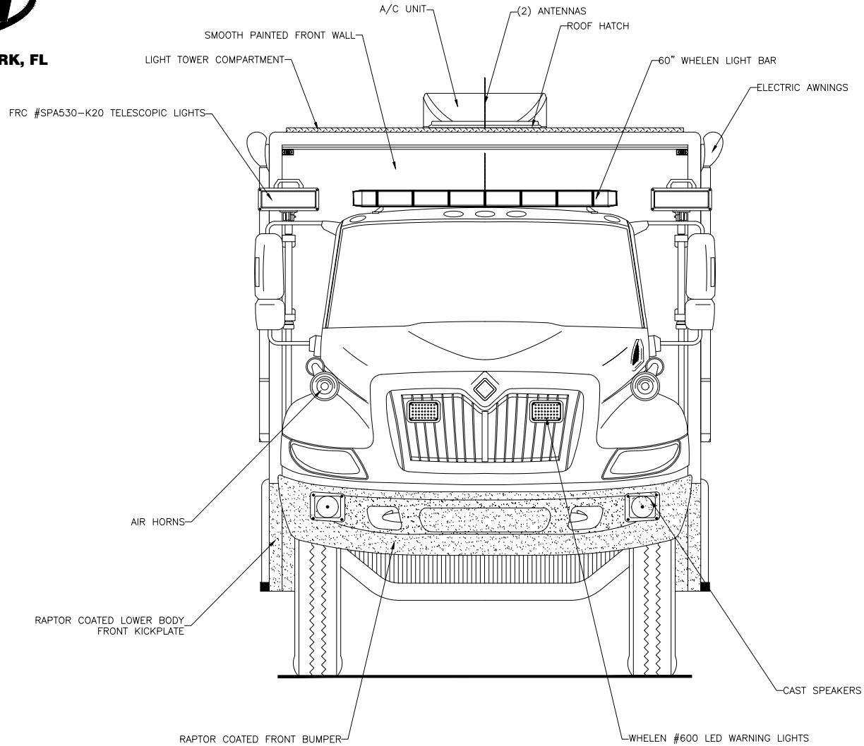
Front View
