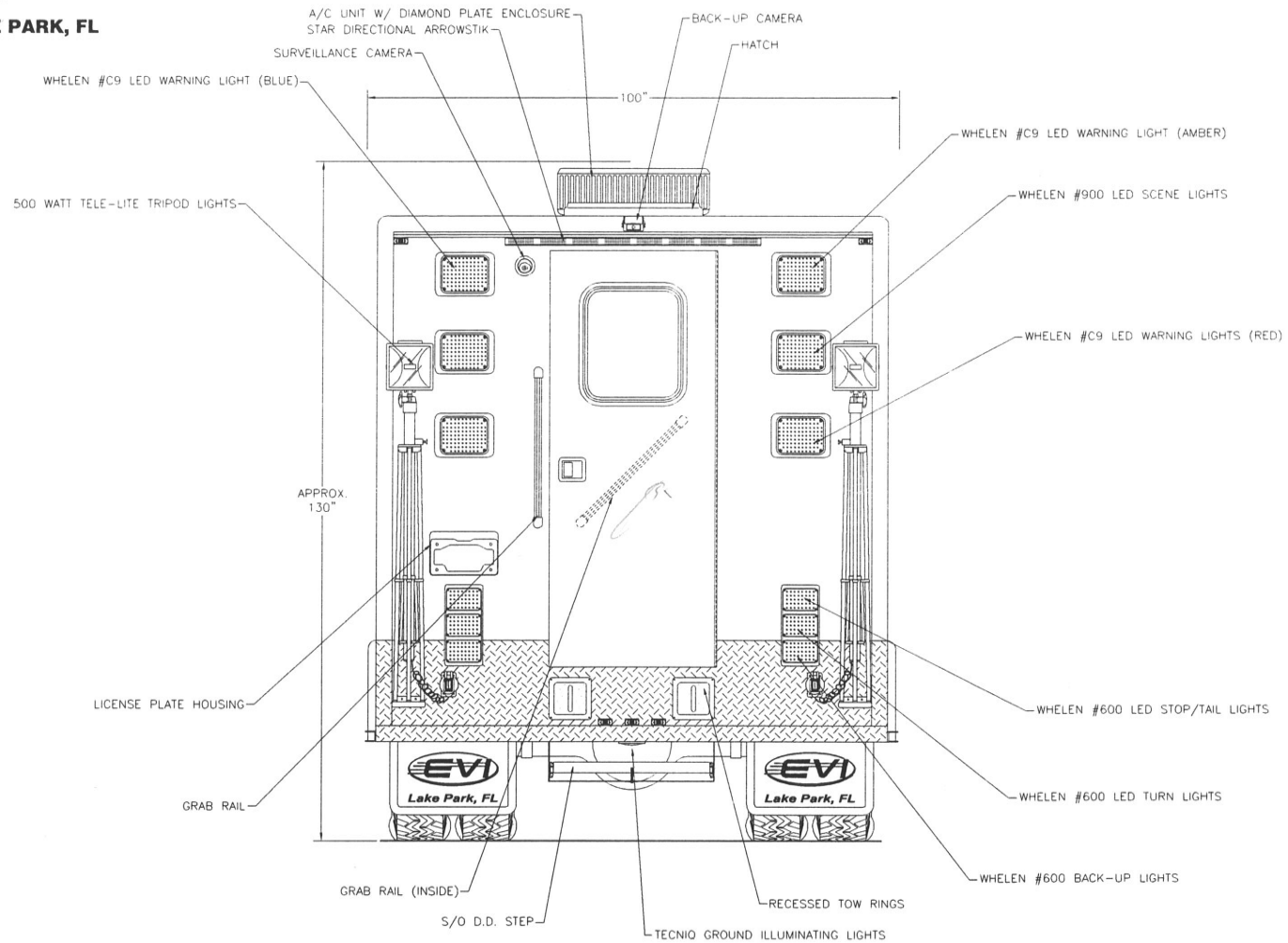
Rear View
